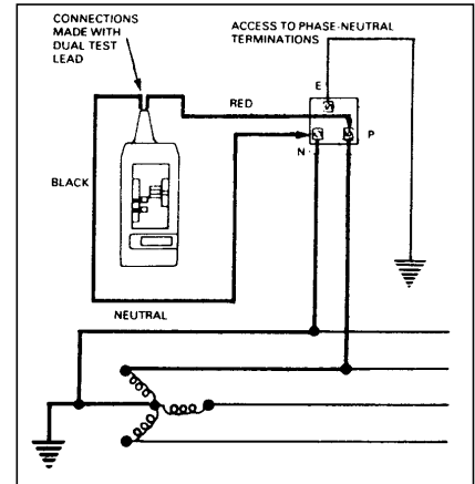
Testing the earth-fault loop impedance of three-phase equipment
