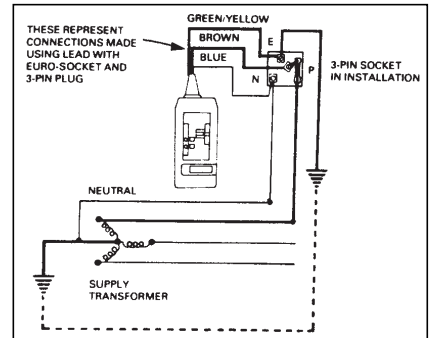
Testing the earth-fault loop impedance at a three-pin socket
