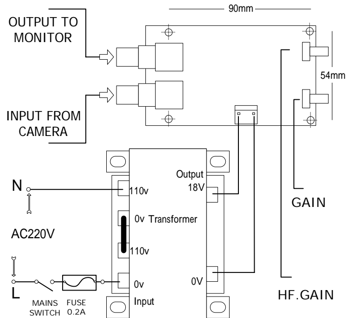
TRANSFORMER: 6VA 18V
