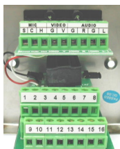
MCN-001 (Female) MCN-002 (Male) VGA+AV+MIC Panel Solder Free Connection Built-in Terminal Blocks Stain-less Steel Panel
