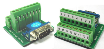
MCN-003 (Female) MCN-004 (Male) VGA Connection Board
