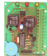
Digital Keypad Module MKP-1100KT Digital Keypad Control Board 2 Programmable Relay Output 3 x 4 Keyboard Not Included Power Source : AC/DC 12V
