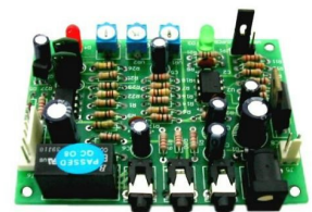
MKT-104 VOX Control Board Microphone Signal Input Mic / Aux Signal Output Contact Output : DPDT Relay Power Source : DC12V ~ 24V
