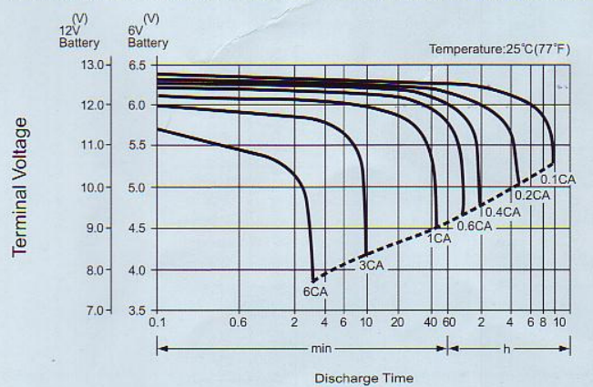
Discharge Characteristic Curves : NPH / NPW / REW Batteries
